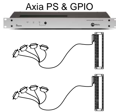
SH+ 4 DB-15M to RJ-21M GPI Break-Out Cable P/N RJ21AXIAGPI-010
