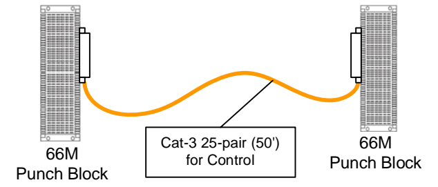
Control Inter-Studio Tie-Lines
