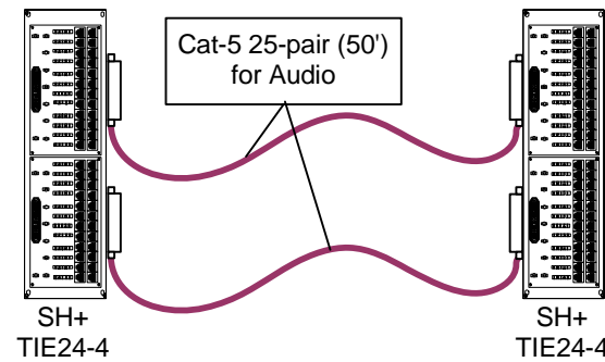
Audio Inter-Studio Tie-Lines
