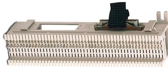
Part # – 11616 66B Block with integrated RJ-21 FEMALE Connector
